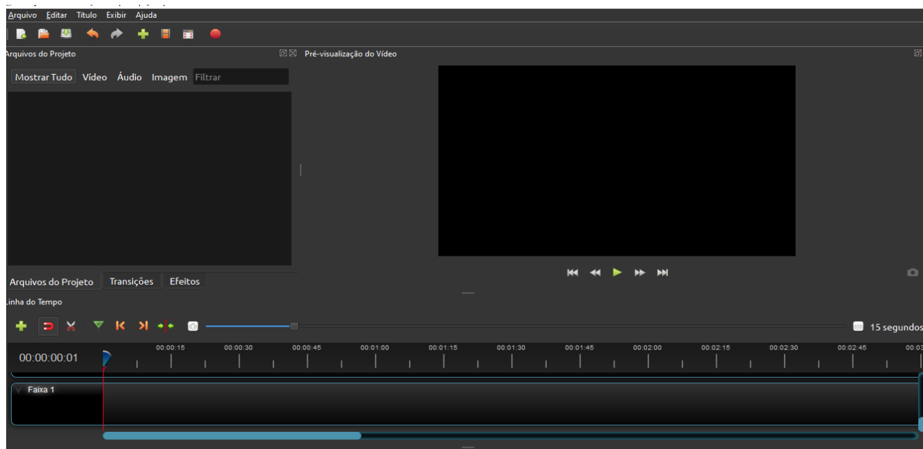
Figura 1 - OpenShot
